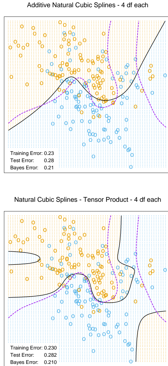
FIGURE 5.11. The simulation example of Figure 2.1. The upper panel shows the decision boundary of an additive logistic regression model, using natural splines in each of the two coordinates (total df = 1 + (4 - 1) + (4 - 1) = 7 ). The lower panel shows the results of using a tensor product of natural spline bases in each coordinate (total df = 4 \times 4 = 16 ). The broken purple boundary is the Bayes decision boundary for this problem.
